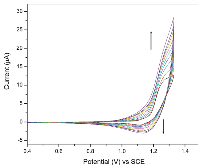
FIGURE 2. Cyclic voltammetry of 5a in CH 2 Cl 2 containing 0.1 M [( n -Bu) 4 N]ClO 4 . Scanned from +0.4 to +1.3 V vs SCE for 10 cycles, scan rate = 100 mV s -1 .
