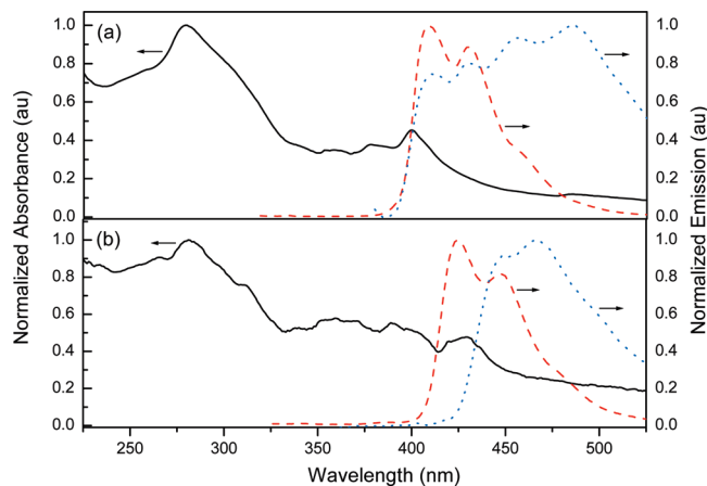
FIGURE 9. (a) Solid-state UV-vis absorption spectrum of 5a (—). Emission spectrum of 5a in solution (---, \lambda_{\text{ex}} = 304 nm) and as a thin film (···, \lambda_{\text{ex}} = 300 nm). (b) Solid-state UV-vis absorption spectrum of 5d (—). Emission spectrum of 5d in solution (---, \lambda_{\text{ex}} = 311 nm) and as a thin film (···, \lambda_{\text{ex}} = 281 nm). All spectra were obtained at ca. 25 °C.
